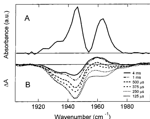
FIGURE 3: (A) Fourier transform infrared spectra of H93G-CO at ambient temperature. The spectra were obtained on a large D 2 O background. The baseline of the background was subtracted to obtain a flat baseline in the region of the three C—O bands observed at 1336, 1445, and 1663 cm -1 . (B) Step-scan FTIR difference spectra showing the CO stretching region at various times after photolysis. The CO stretching frequency at equilibrium is shown in the top spectrum. Difference spectra are shown at 125 \mu s, 250 \mu s, 375 \mu s, 500 \mu s, 1 ms, and 4 ms.
